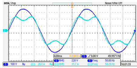
Low harmonics
