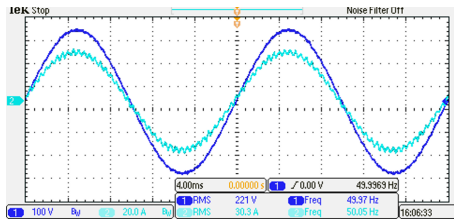
High harmonics
